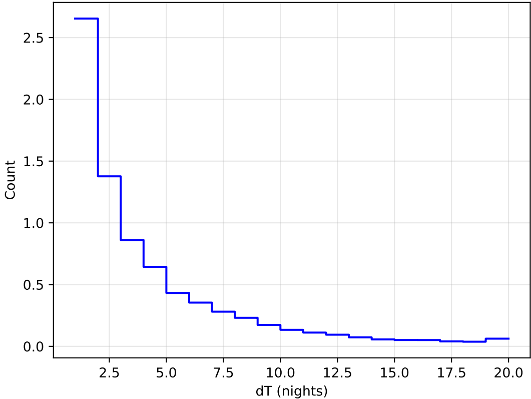
ddf_loaded_fl15_v3.4_10yrs WFD all bands: DeltaNight Histogram 1e6
