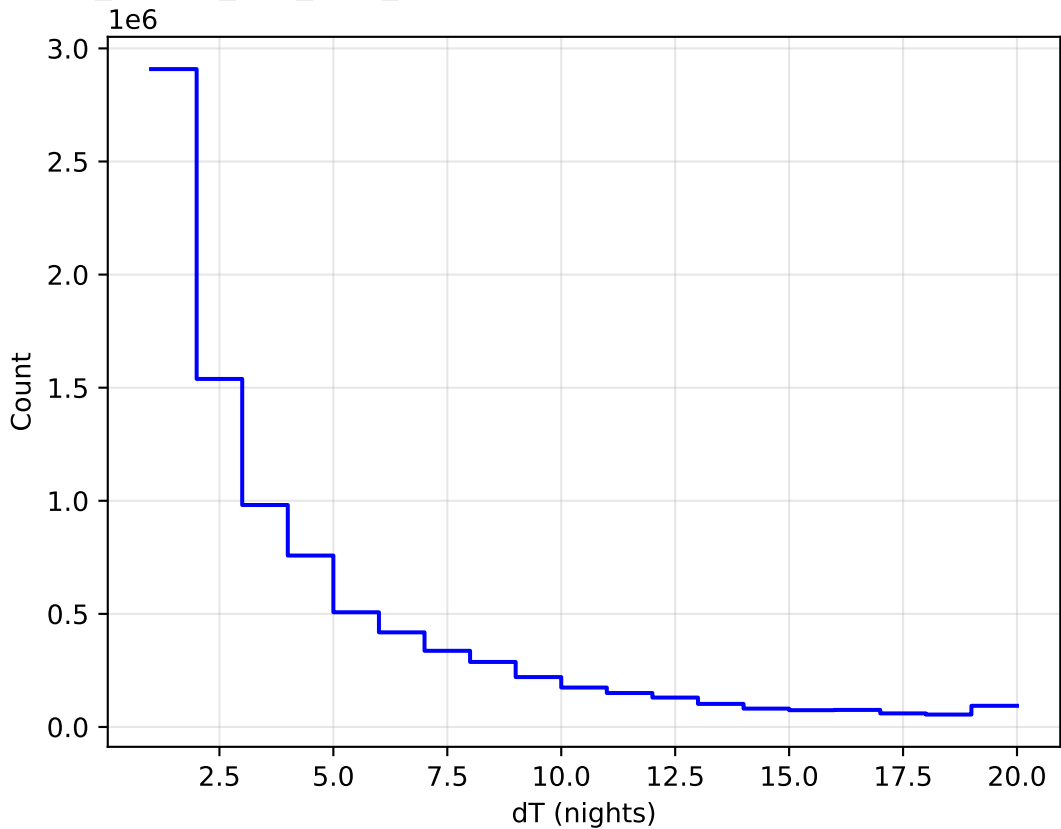
ddf_loaded_fl15_v3.4_10yrs All sky all bands: DeltaNight Histogram
