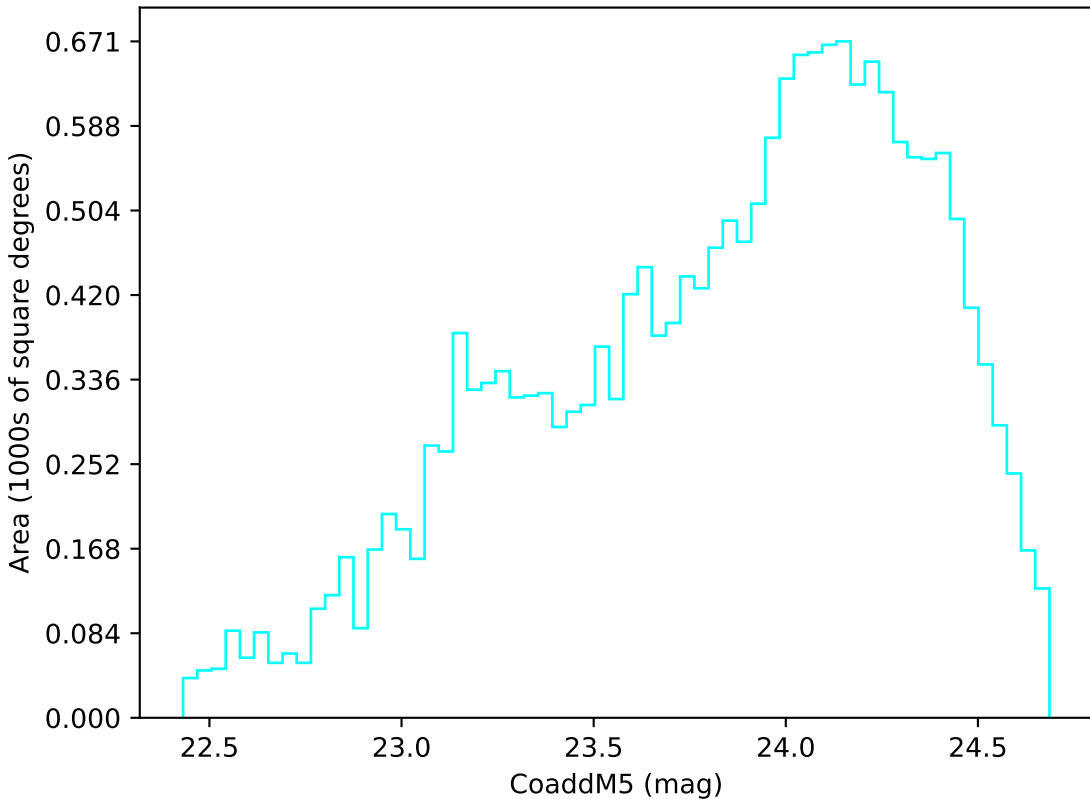
ddf_loaded_fl15_v3.4_10yrs Yr 3-4 u band: CoaddM5
