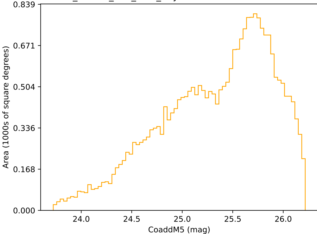
ddf_loaded_fl15_v3.4_10yrs Yr 3-4 r band: CoaddM5
