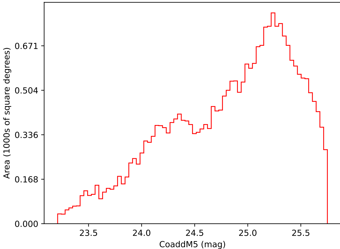
ddf_loaded_fl15_v3.4_10yrs Yr 3-4 i band: CoaddM5
