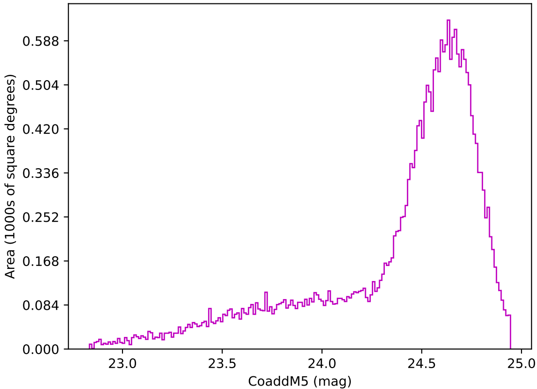
ddf_loaded_fl15_v3.4_10yrs Yr 1 z band: CoaddM5
