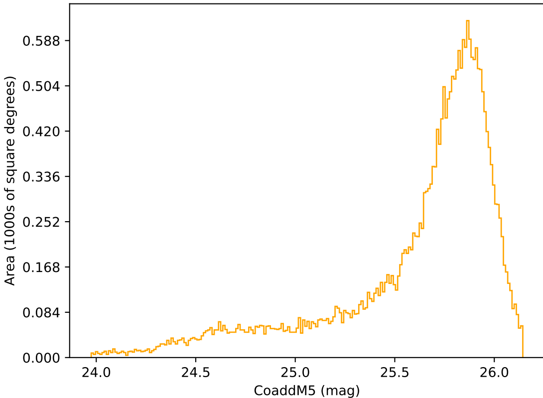
ddf_loaded_fl15_v3.4_10yrs Yr 1 r band: CoaddM5
