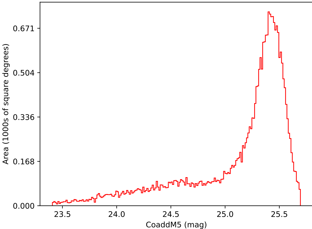
ddf_loaded_fl15_v3.4_10yrs Yr 1 i band: CoaddM5
