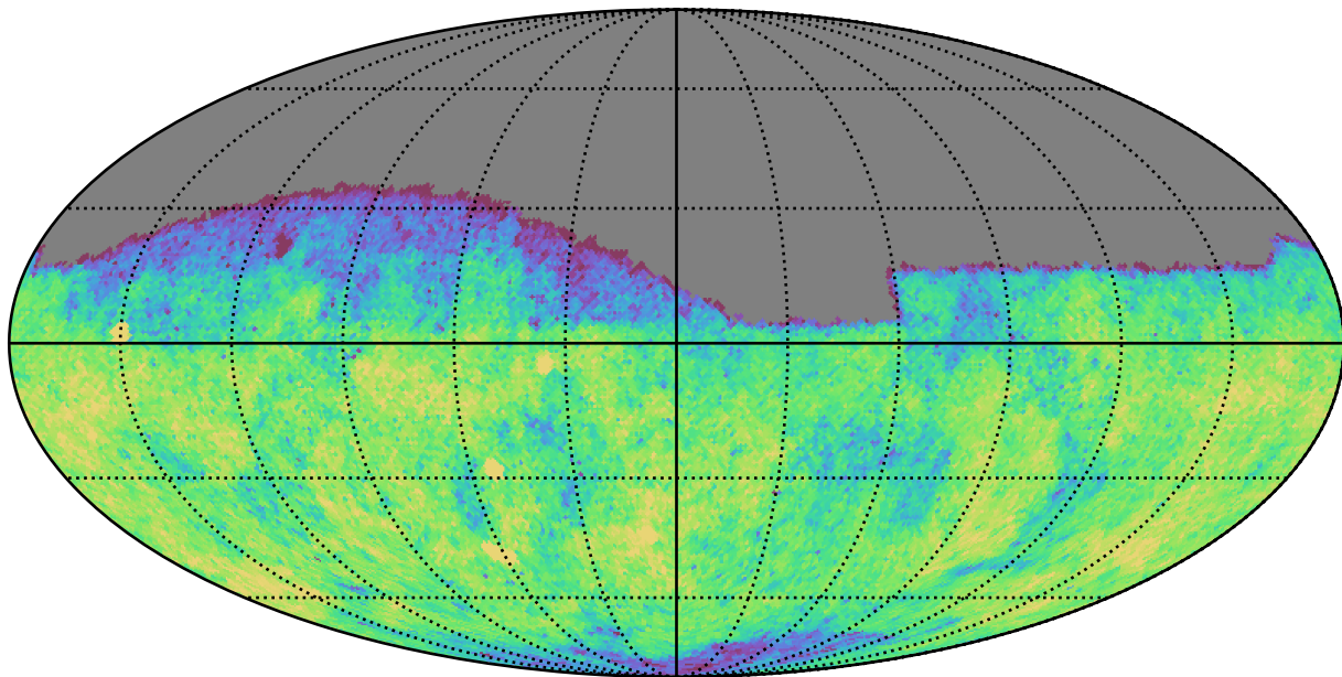
ddf_loaded_fl15_v3.4_10yrs Yr 1 g band: CoaddM5
