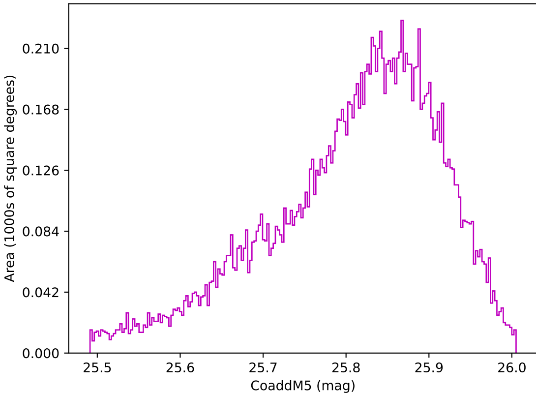
ddf_loaded_fl15_v3.4_10yrs WFD z band: CoaddM5
