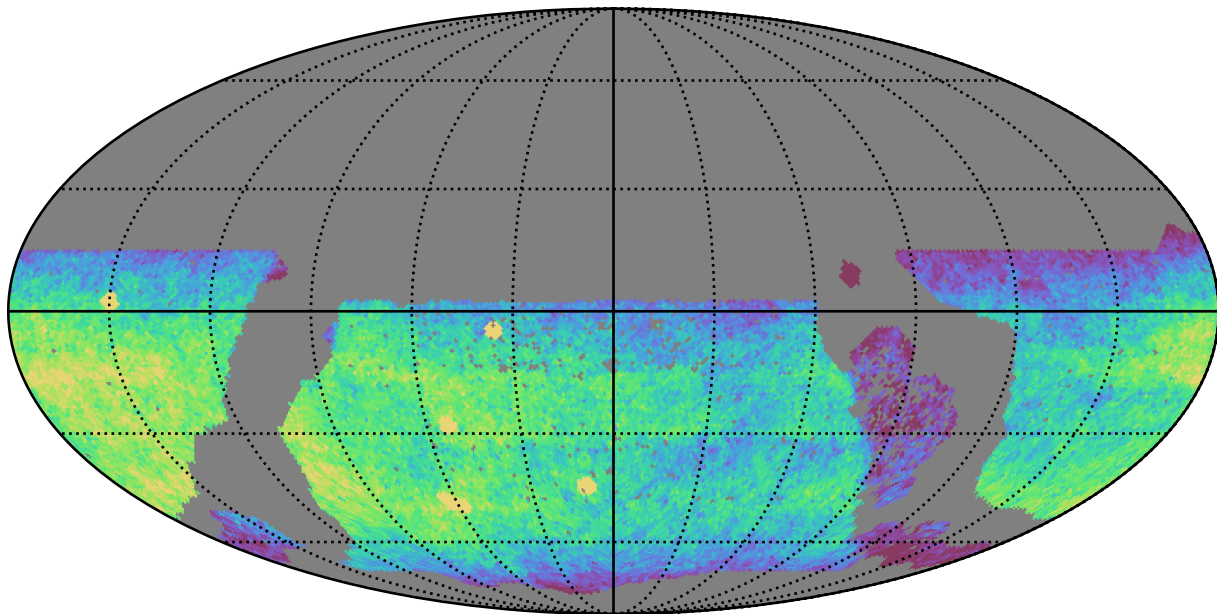
ddf_loaded_fl15_v3.4_10yrs WFD u band: CoaddM5
