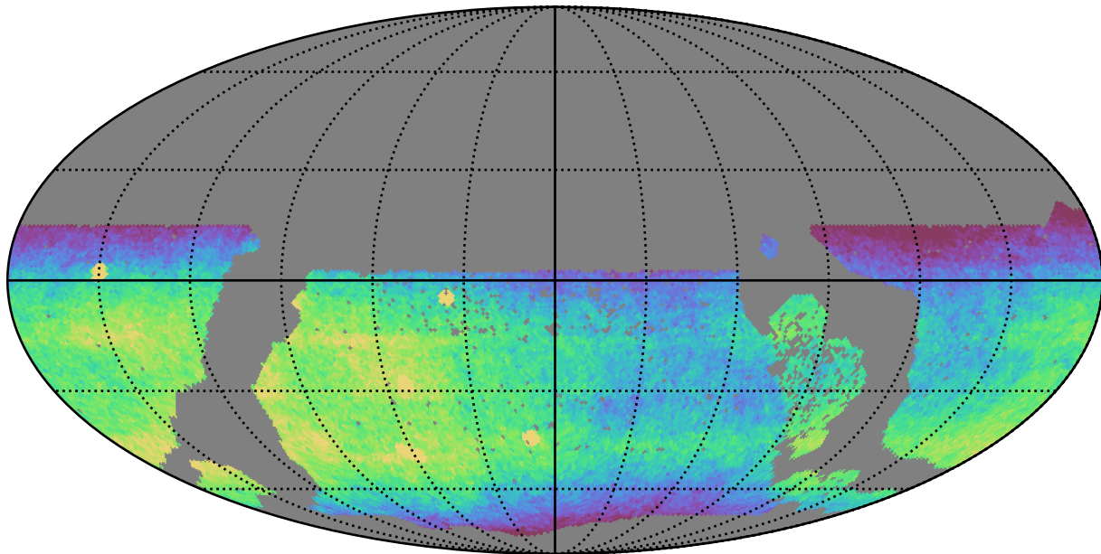
ddf_loaded_fl15_v3.4_10yrs WFD r band: CoaddM5
