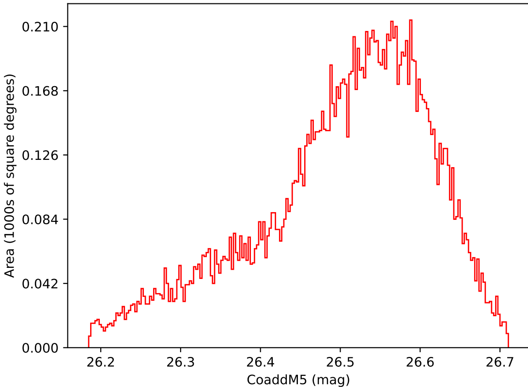
ddf_loaded_fl15_v3.4_10yrs WFD i band: CoaddM5
