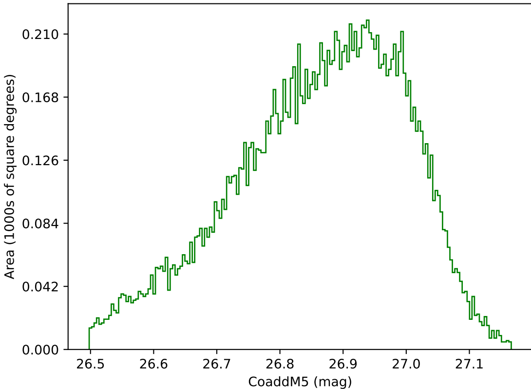
ddf_loaded_fl15_v3.4_10yrs WFD g band: CoaddM5
