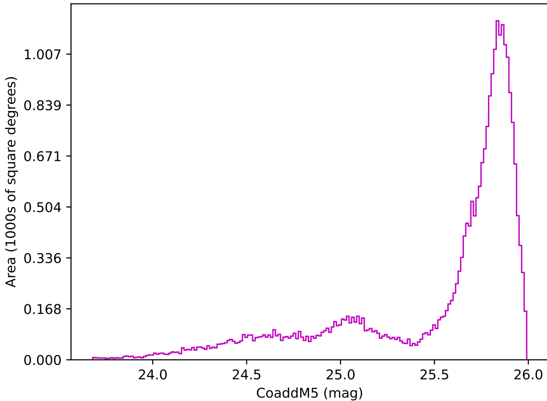
ddf_loaded_fl15_v3.4_10yrs All sky z band: CoaddM5
