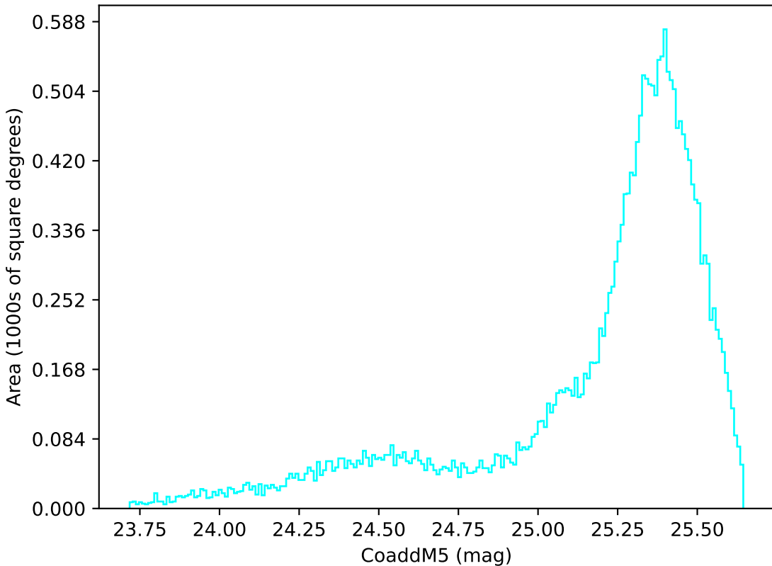
ddf_loaded_fl15_v3.4_10yrs All sky u band: CoaddM5
