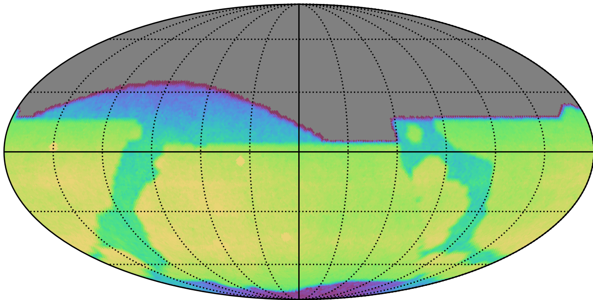
ddf_loaded_fl15_v3.4_10yrs All sky r band: CoaddM5
