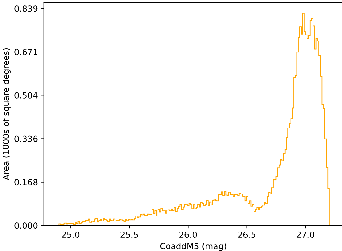
ddf_loaded_fl15_v3.4_10yrs All sky r band: CoaddM5
