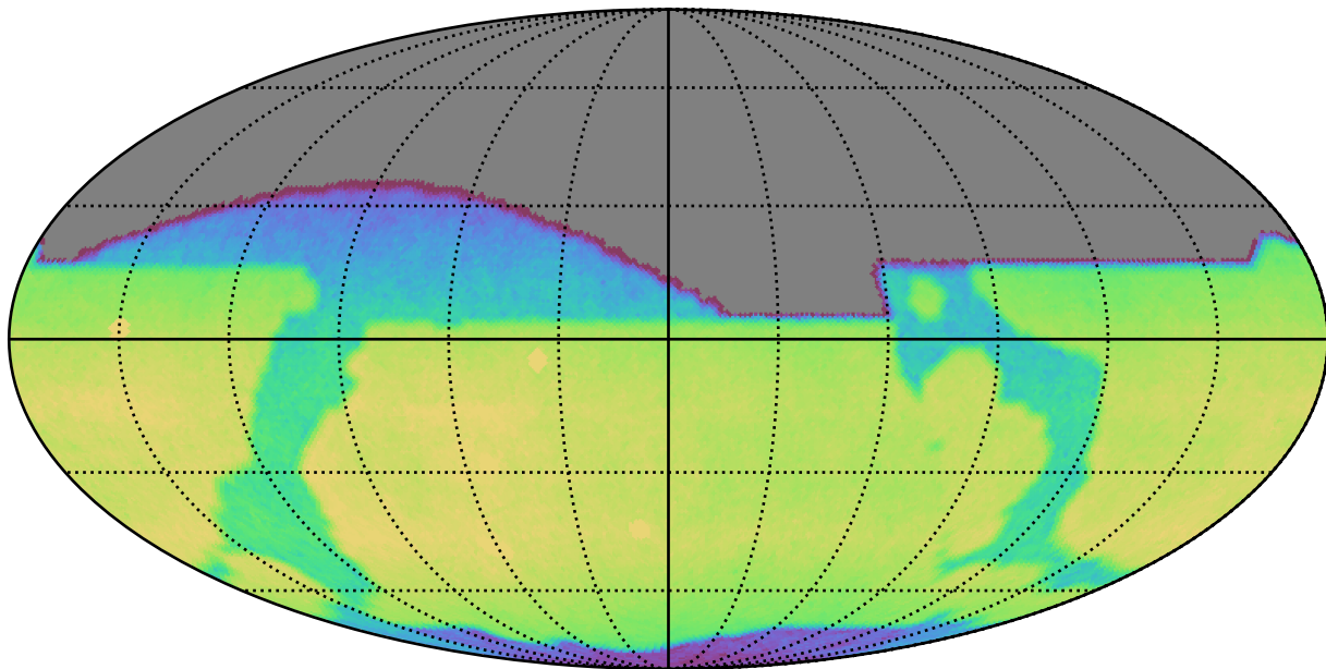
ddf_loaded_fl15_v3.4_10yrs All sky i band: CoaddM5
