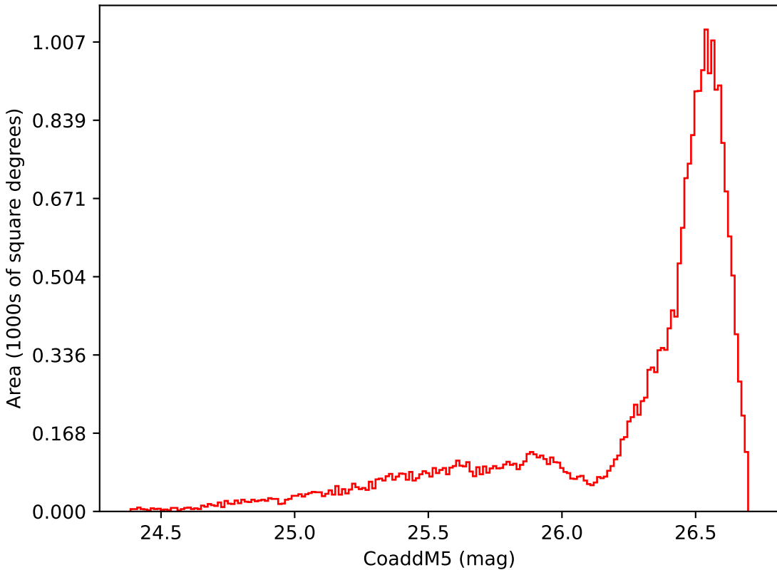
ddf_loaded_fl15_v3.4_10yrs All sky i band: CoaddM5
