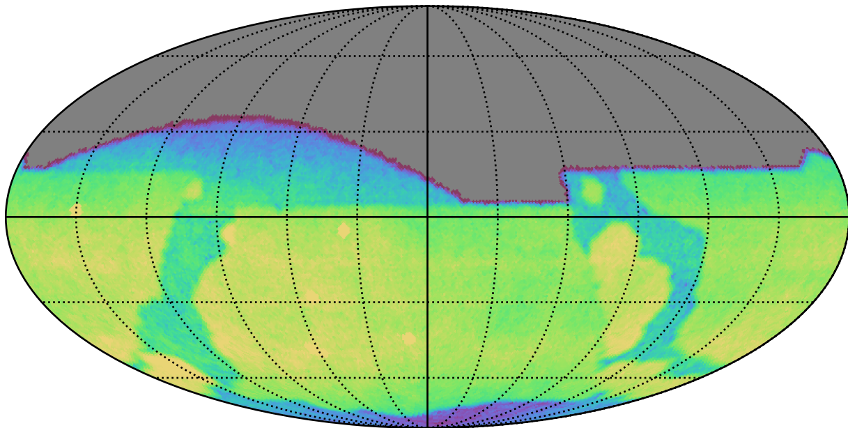
ddf_loaded_fl15_v3.4_10yrs All sky g band: CoaddM5
