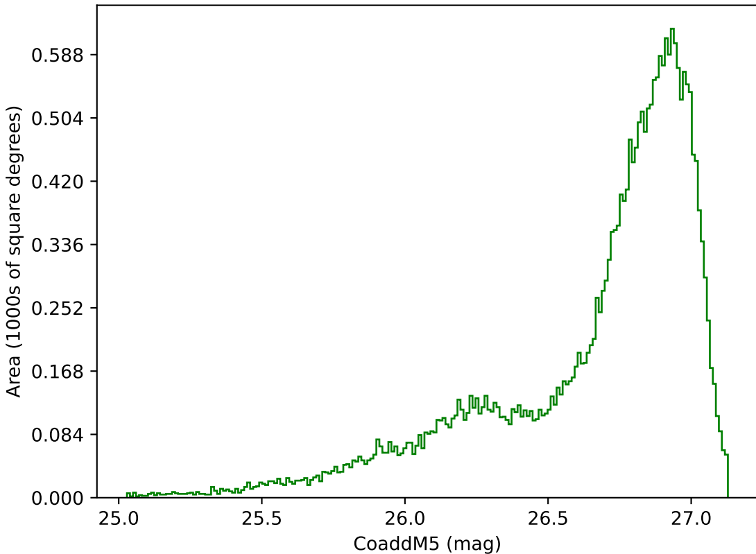
ddf_loaded_fl15_v3.4_10yrs All sky g band: CoaddM5
