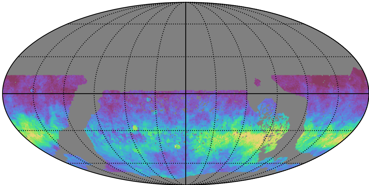
ddf_loaded_fl15_v3.4_10yrs WFD z band: AngleRms rotSkyPos
