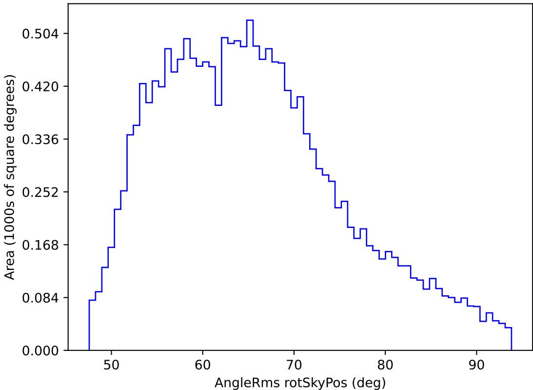
ddf_loaded_fl15_v3.4_10yrs WFD z band: AngleRms rotSkyPos
