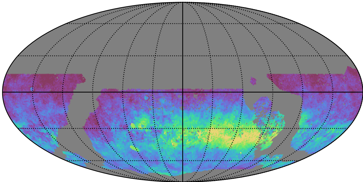
ddf_loaded_fl15_v3.4_10yrs WFD y band: AngleRms rotSkyPos
