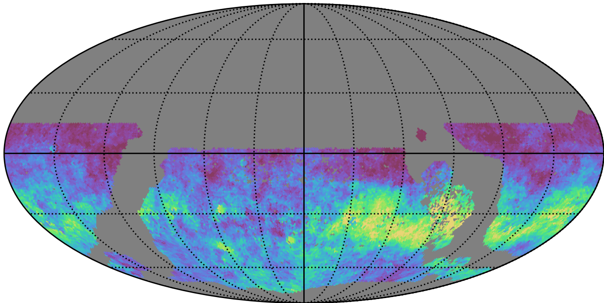
ddf_loaded_fl15_v3.4_10yrs WFD u band: AngleRms rotSkyPos
