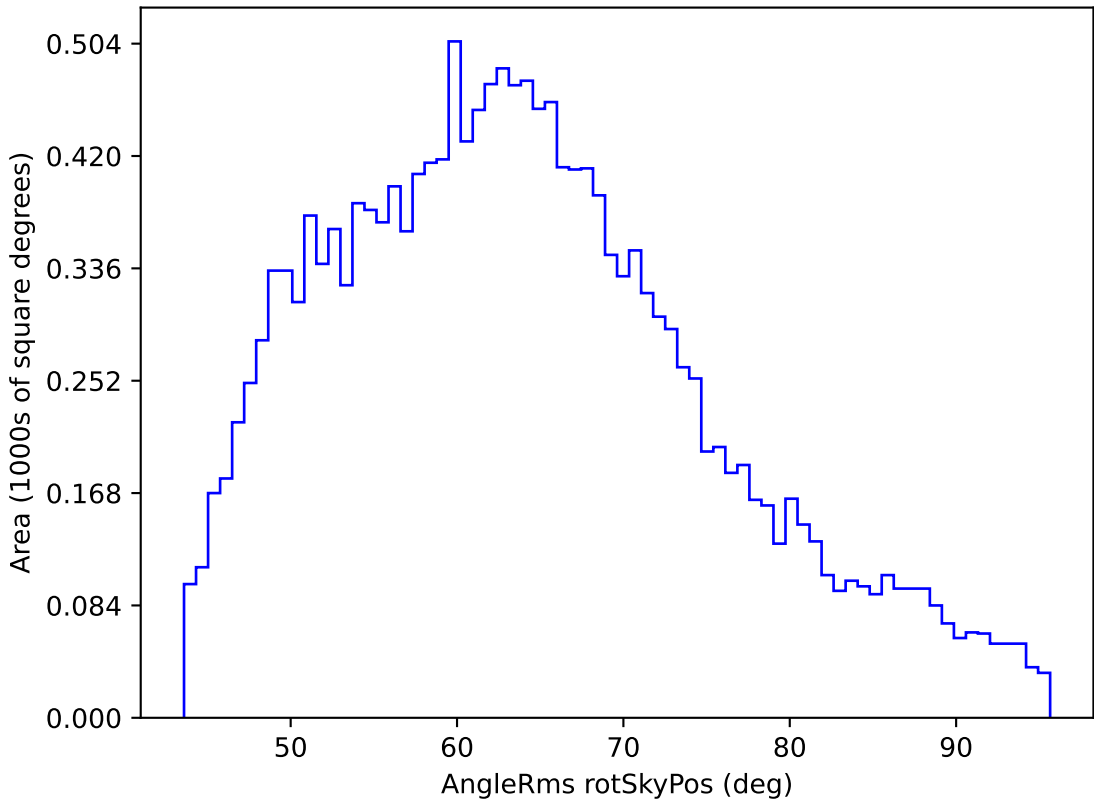
ddf_loaded_fl15_v3.4_10yrs WFD u band: AngleRms rotSkyPos
