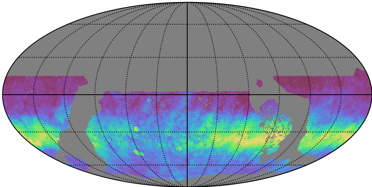
ddf_loaded_fl15_v3.4_10yrs WFD r band: AngleRms rotSkyPos
