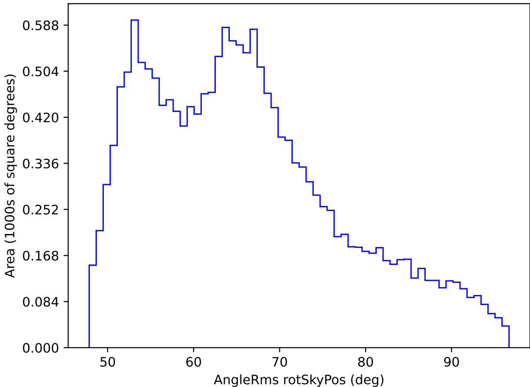
ddf_loaded_fl15_v3.4_10yrs WFD r band: AngleRms rotSkyPos
