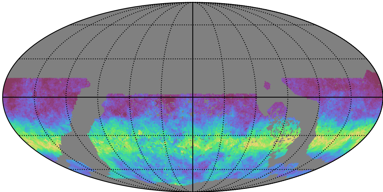
ddf_loaded_fl15_v3.4_10yrs WFD g band: AngleRms rotSkyPos
