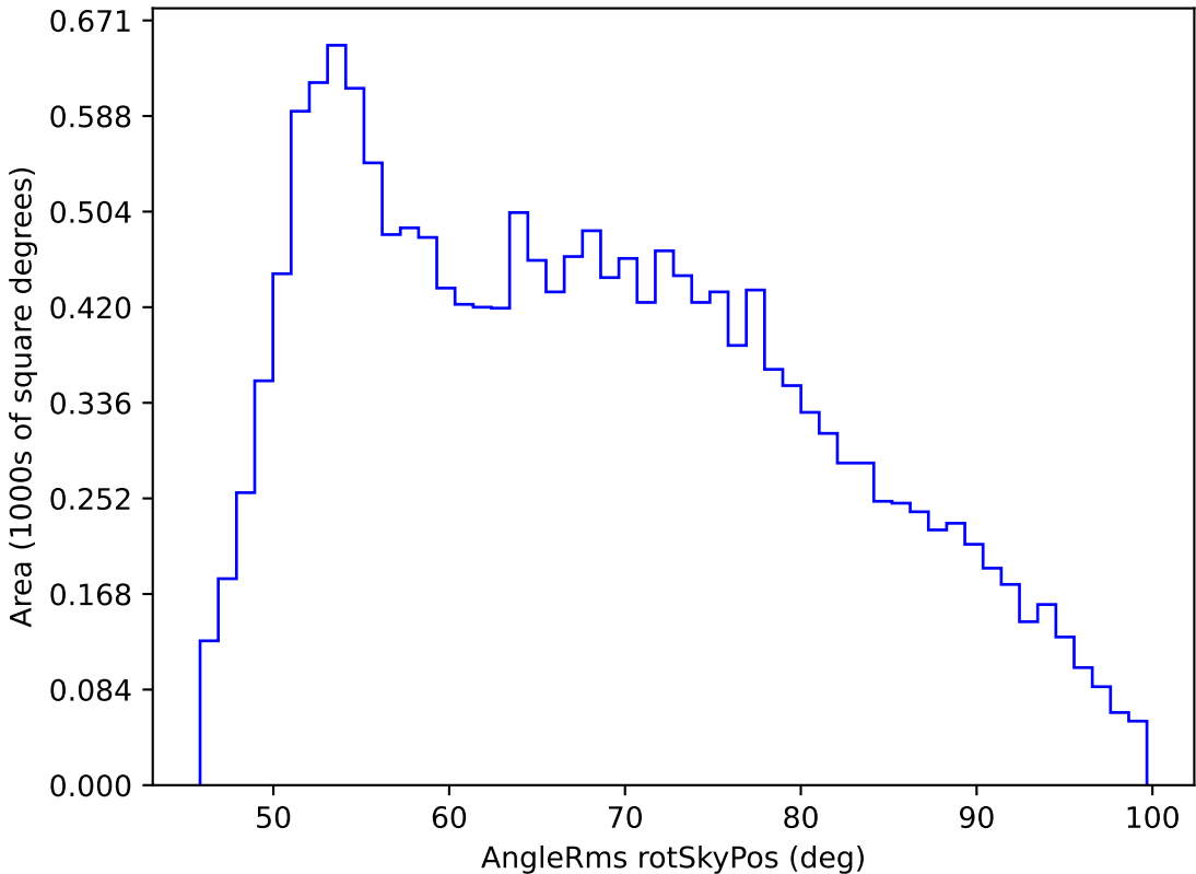
ddf_loaded_fl15_v3.4_10yrs WFD g band: AngleRms rotSkyPos
