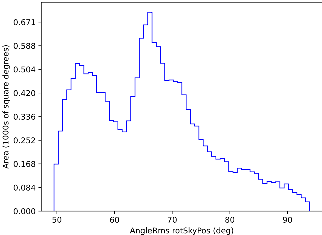
ddf_loaded_fl15_v3.4_10yrs WFD all bands: AngleRms rotSkyPos
