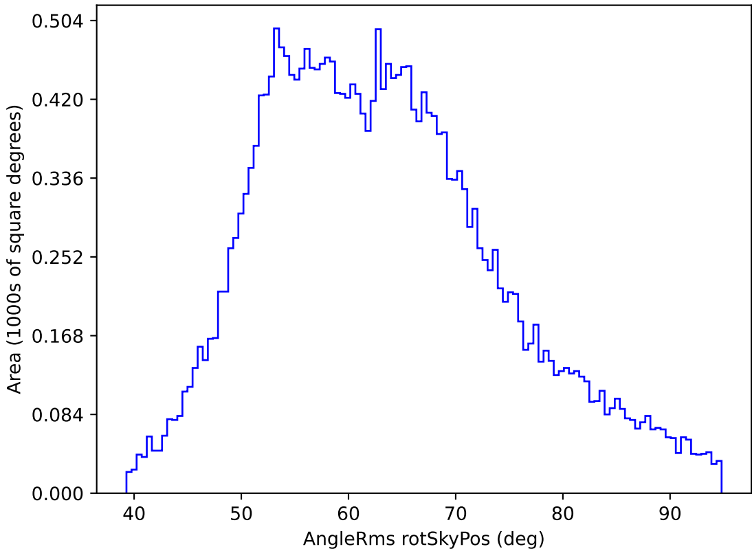
ddf_loaded_fl15_v3.4_10yrs All sky z band: AngleRms rotSkyPos
