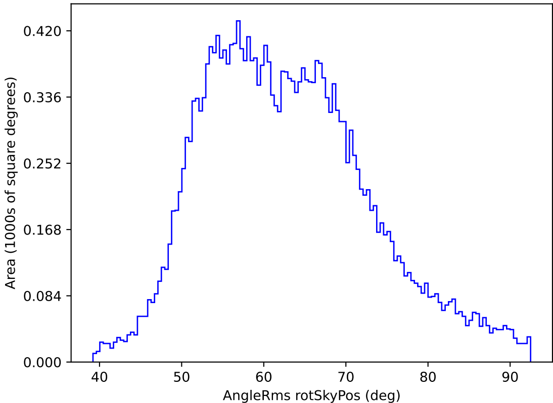
ddf_loaded_fl15_v3.4_10yrs All sky y band: AngleRms rotSkyPos
