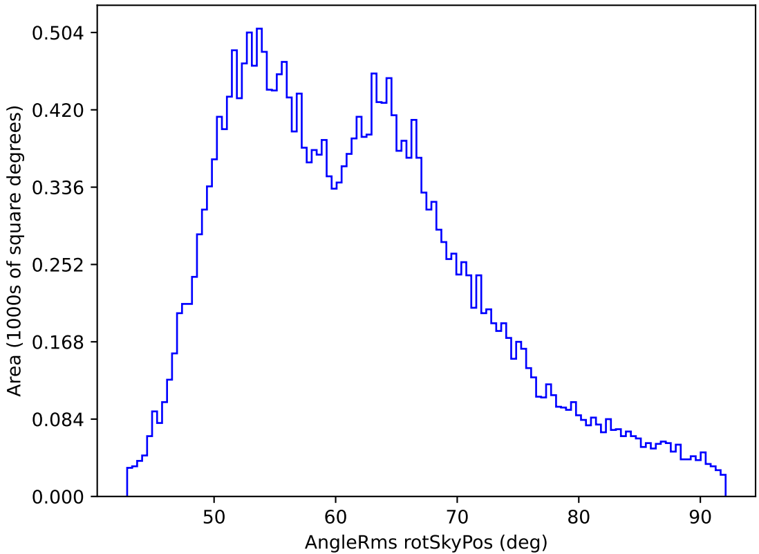
ddf_loaded_fl15_v3.4_10yrs All sky i band: AngleRms rotSkyPos
