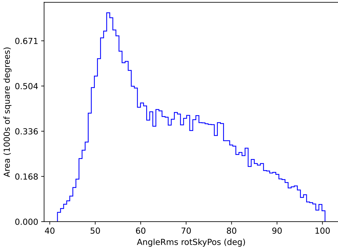
ddf_loaded_fl15_v3.4_10yrs All sky g band: AngleRms rotSkyPos
