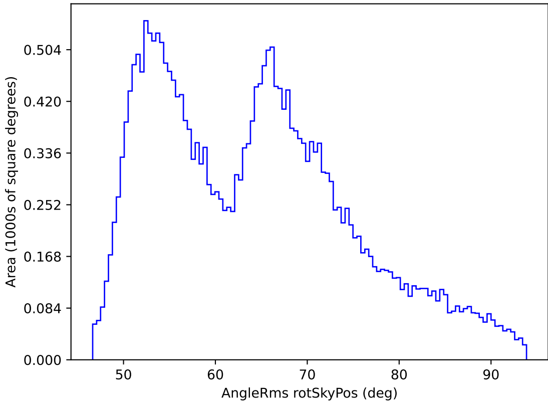
ddf_loaded_fl15_v3.4_10yrs All sky all bands: AngleRms rotSkyPos
