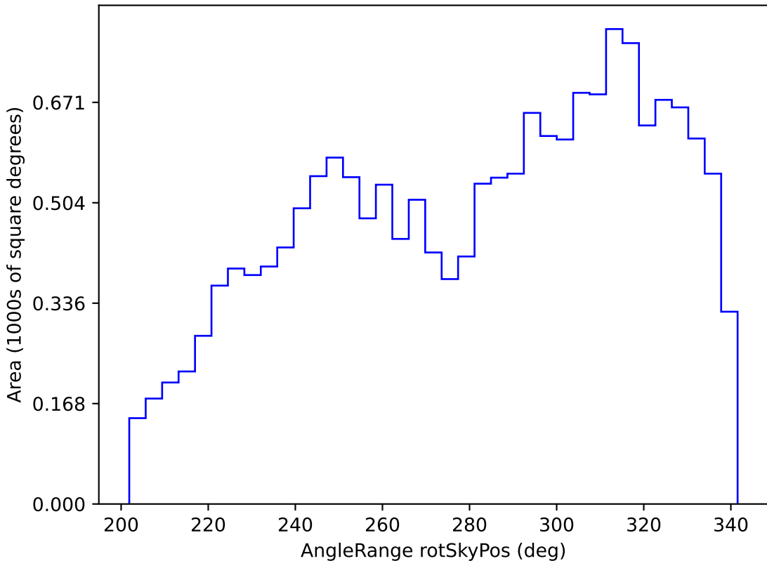
ddf_loaded_fl15_v3.4_10yrs WFD z band: AngleRange rotSkyPos
