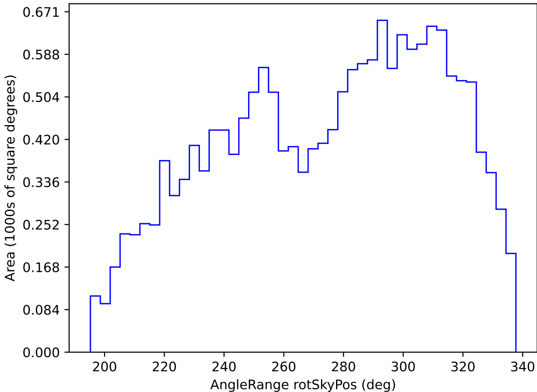
ddf_loaded_fl15_v3.4_10yrs WFD y band: AngleRange rotSkyPos
