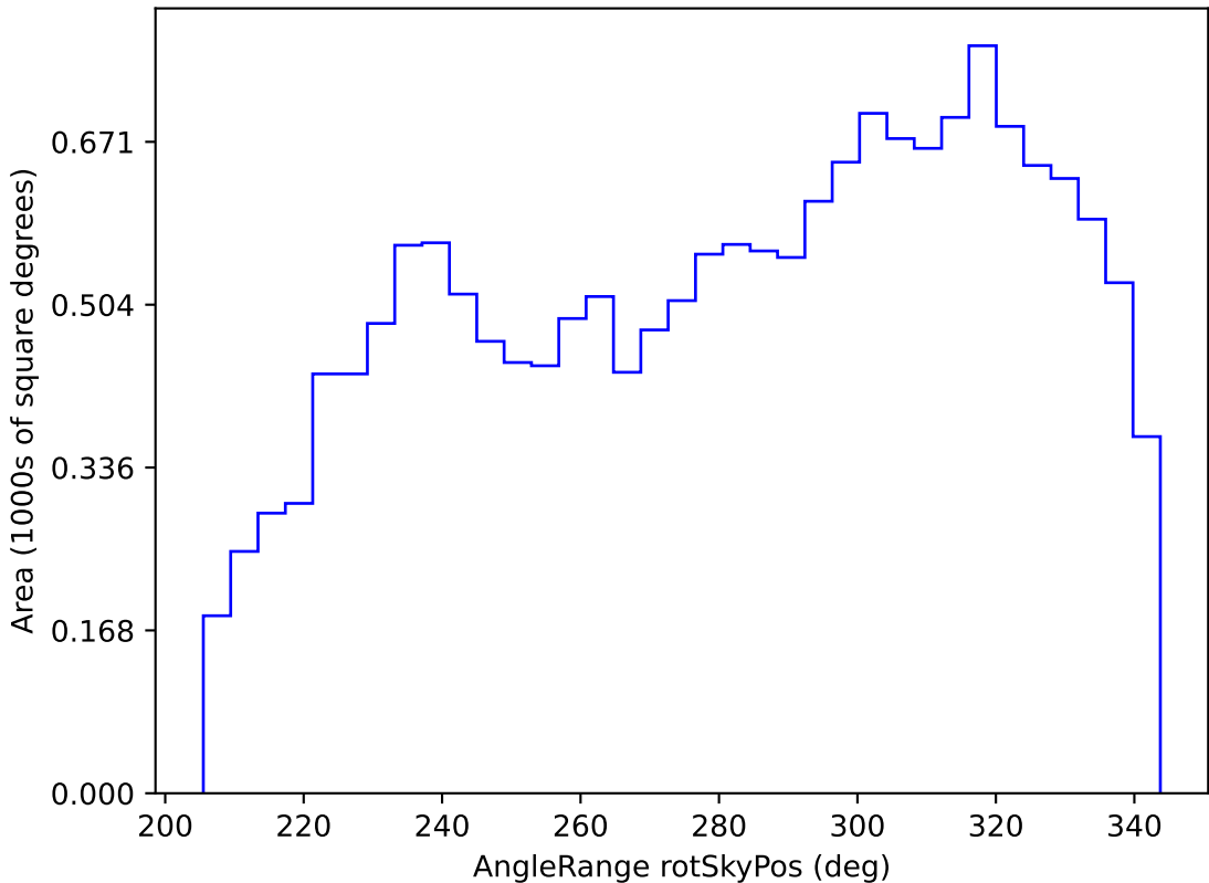
ddf_loaded_fl15_v3.4_10yrs WFD r band: AngleRange rotSkyPos
