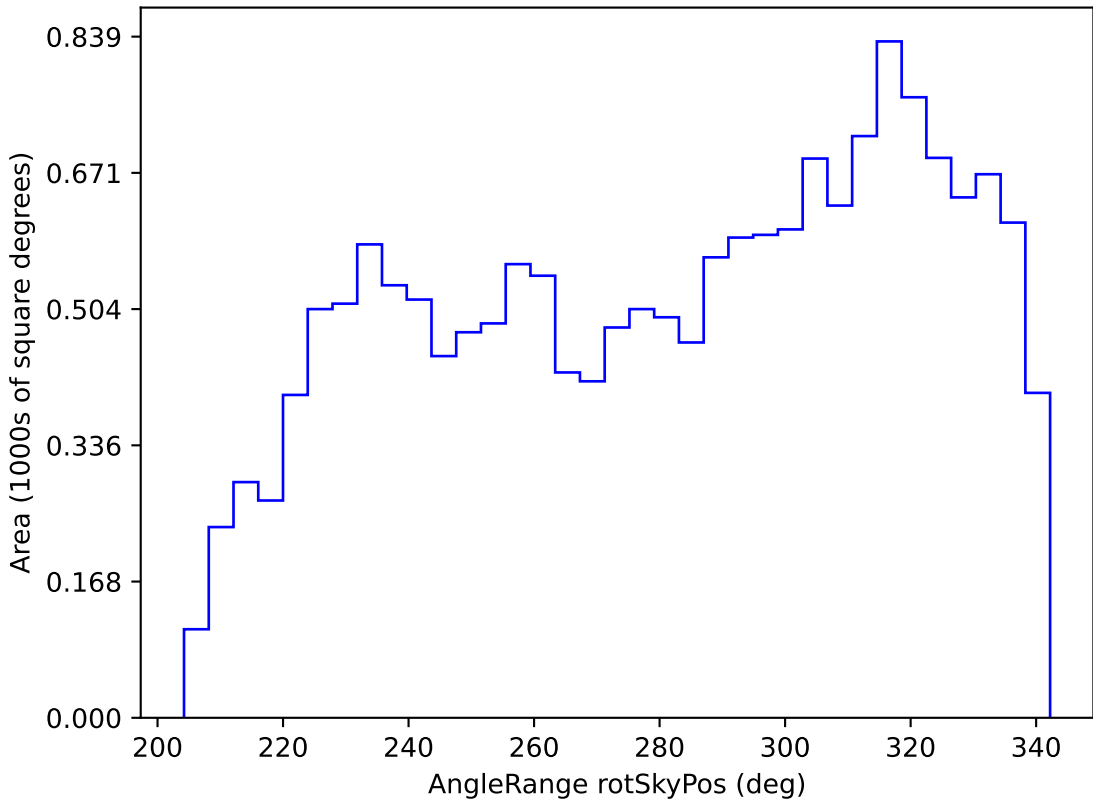
ddf_loaded_fl15_v3.4_10yrs WFD i band: AngleRange rotSkyPos
