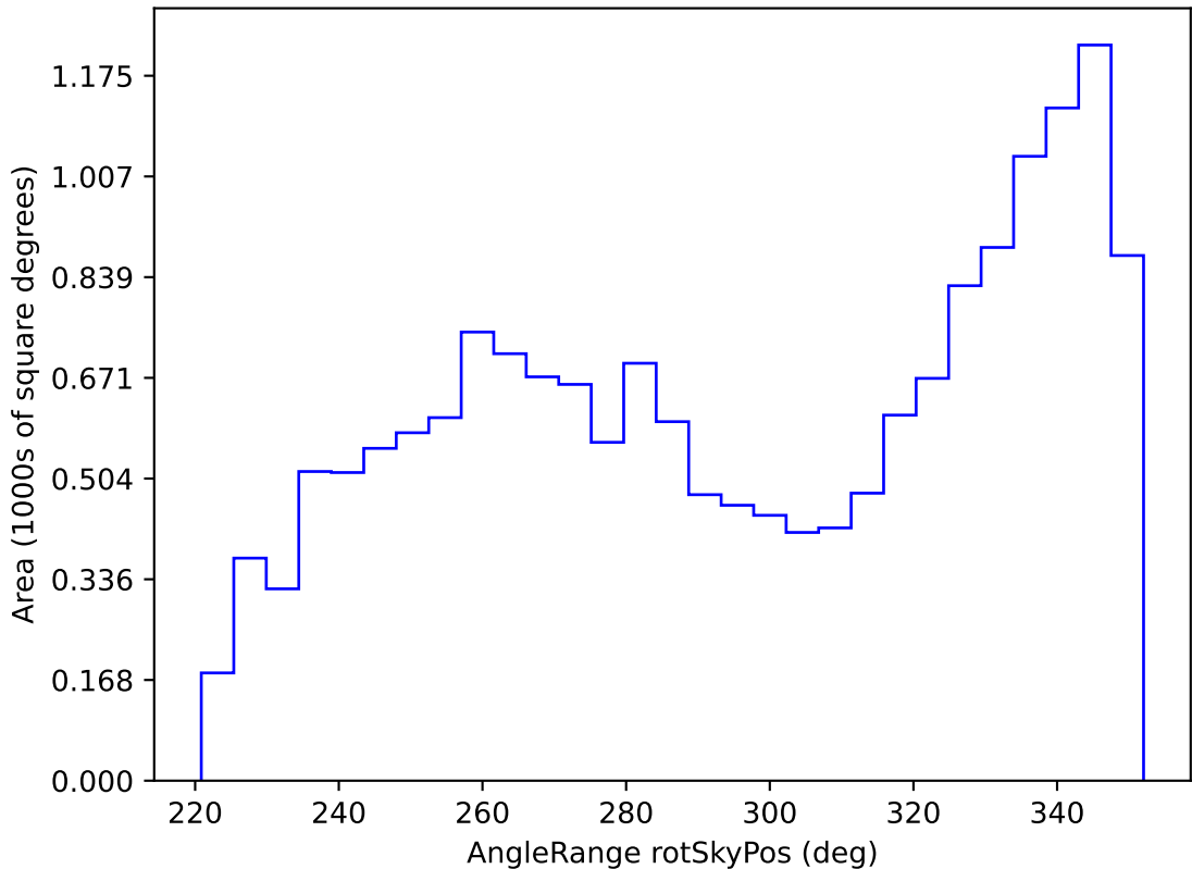
ddf_loaded_fl15_v3.4_10yrs WFD all bands: AngleRange rotSkyPos
