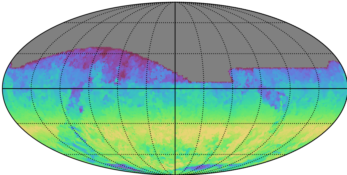
ddf_loaded_fl15_v3.4_10yrs All sky z band: AngleRange rotSkyPos
