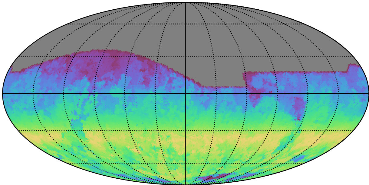
ddf_loaded_fl15_v3.4_10yrs All sky r band: AngleRange rotSkyPos
