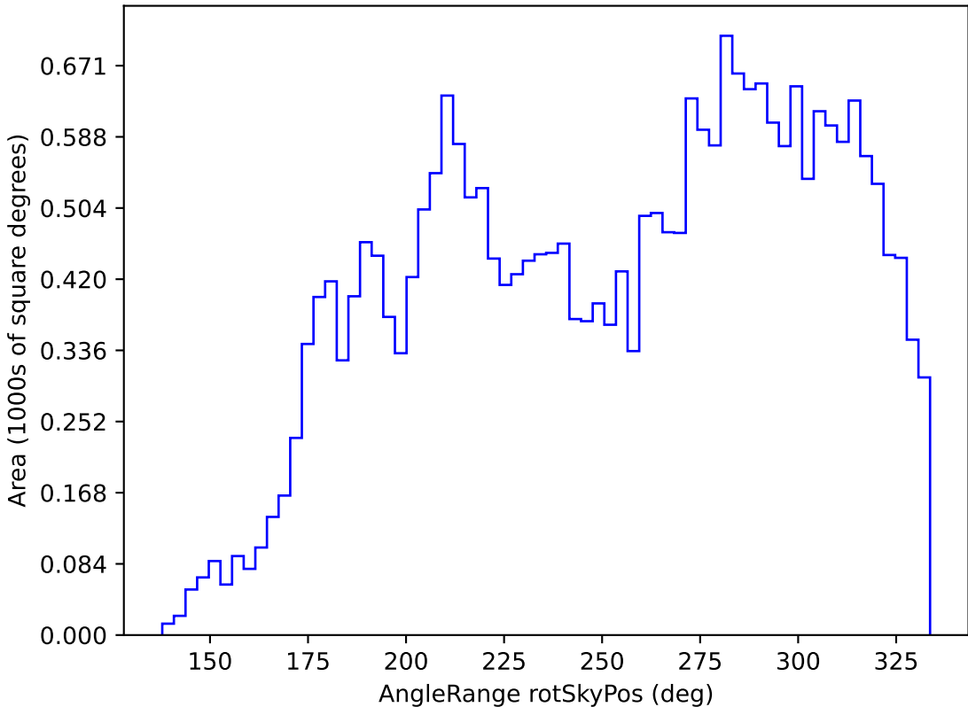
ddf_loaded_fl15_v3.4_10yrs All sky g band: AngleRange rotSkyPos
