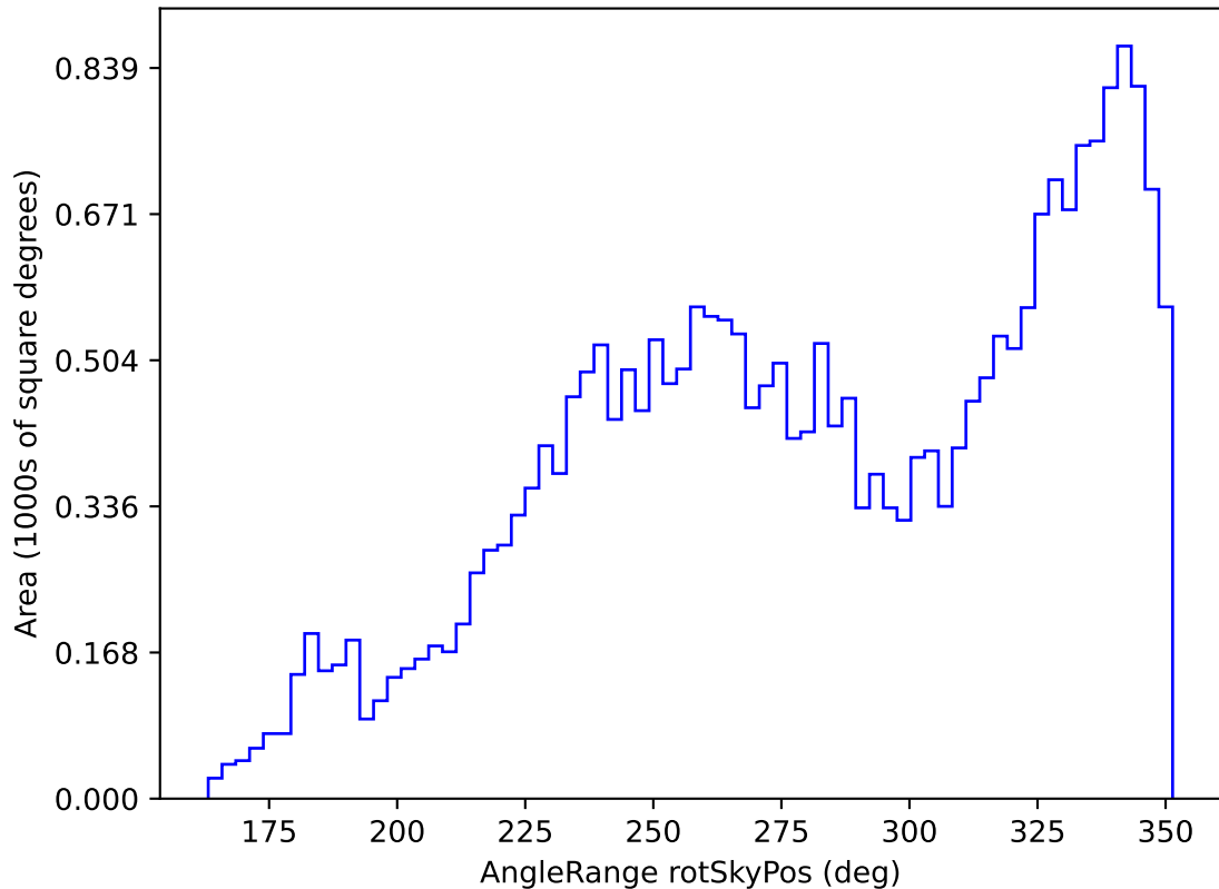
ddf_loaded_fl15_v3.4_10yrs All sky all bands: AngleRange rotSkyPos
