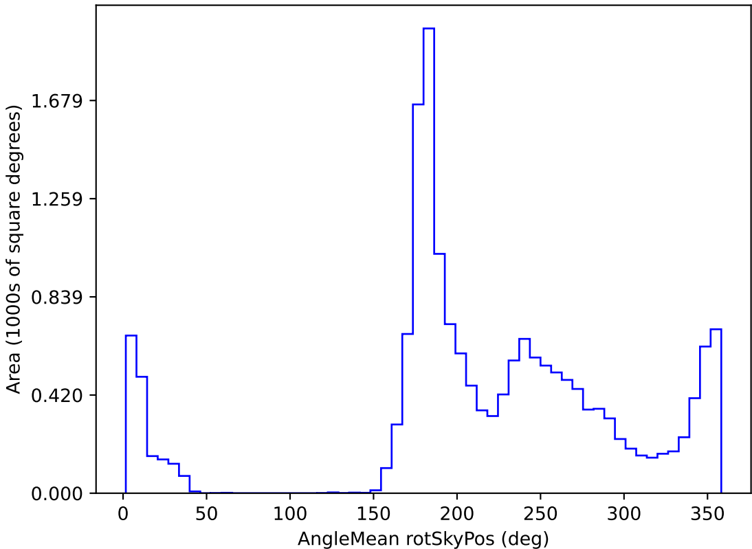
ddf_loaded_fl15_v3.4_10yrs WFD z band: AngleMean rotSkyPos
