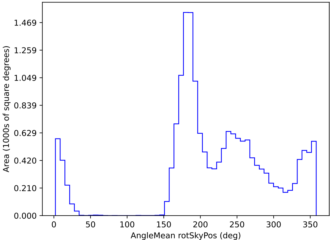
ddf_loaded_fl15_v3.4_10yrs WFD y band: AngleMean rotSkyPos
