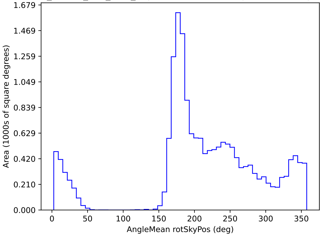
ddf_loaded_fl15_v3.4_10yrs WFD u band: AngleMean rotSkyPos
