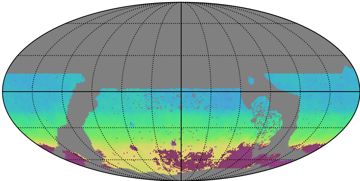
ddf_loaded_fl15_v3.4_10yrs WFD i band: AngleMean rotSkyPos
